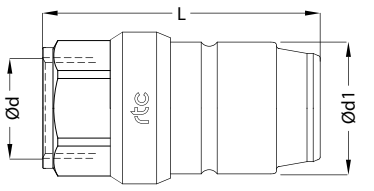
Plug Profile: 152.32 - 152.38 - 152.50
